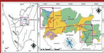
Southern Granulite Terrain
