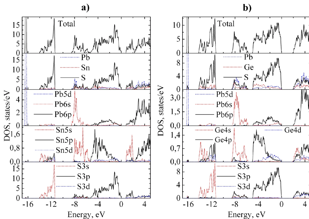
Fig. 5. Total and partial densities of states of \text{PbSnS}_3 (a) and \text{PbGeS}_3 (b).
